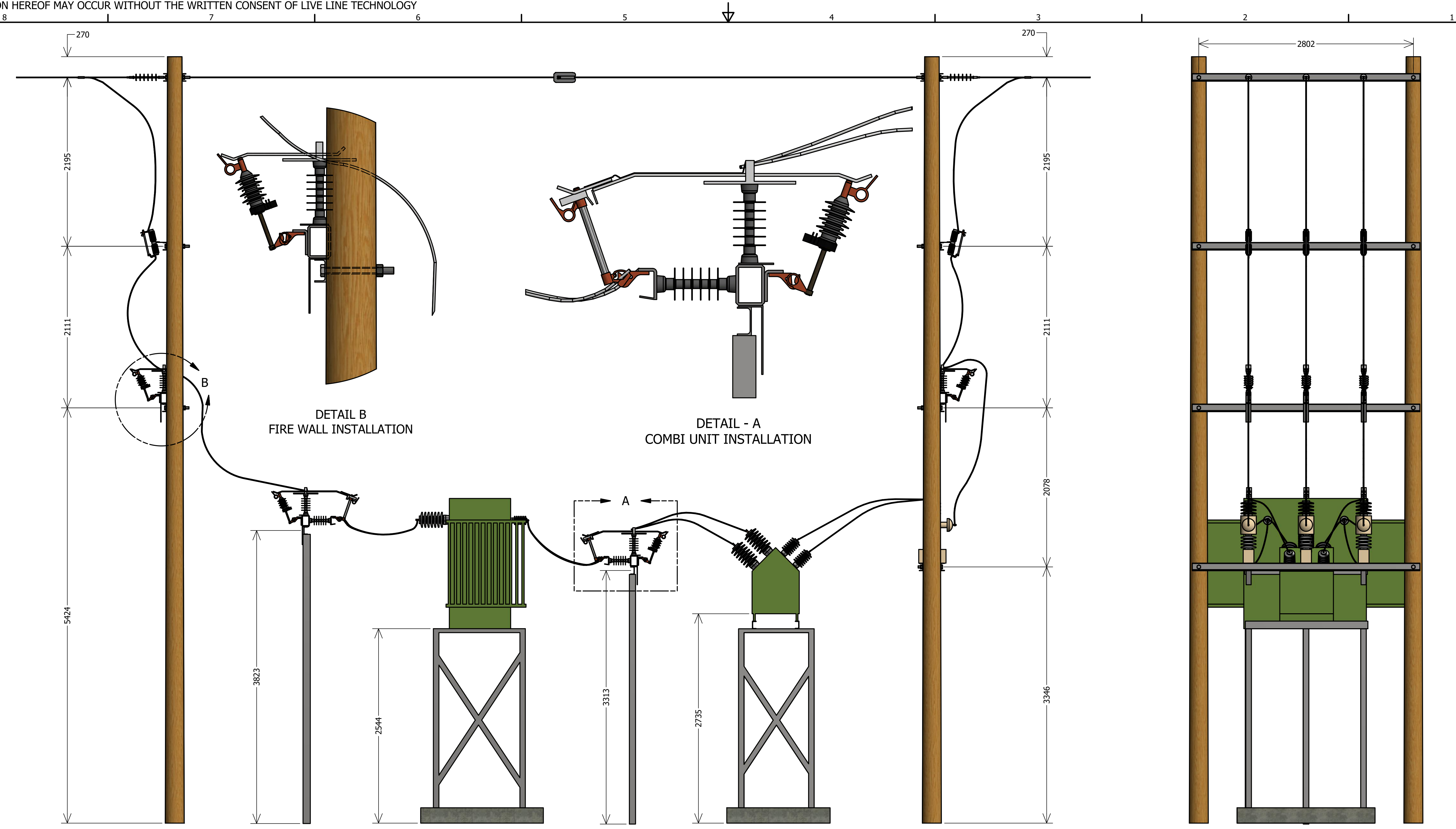
SIDE VIEW
