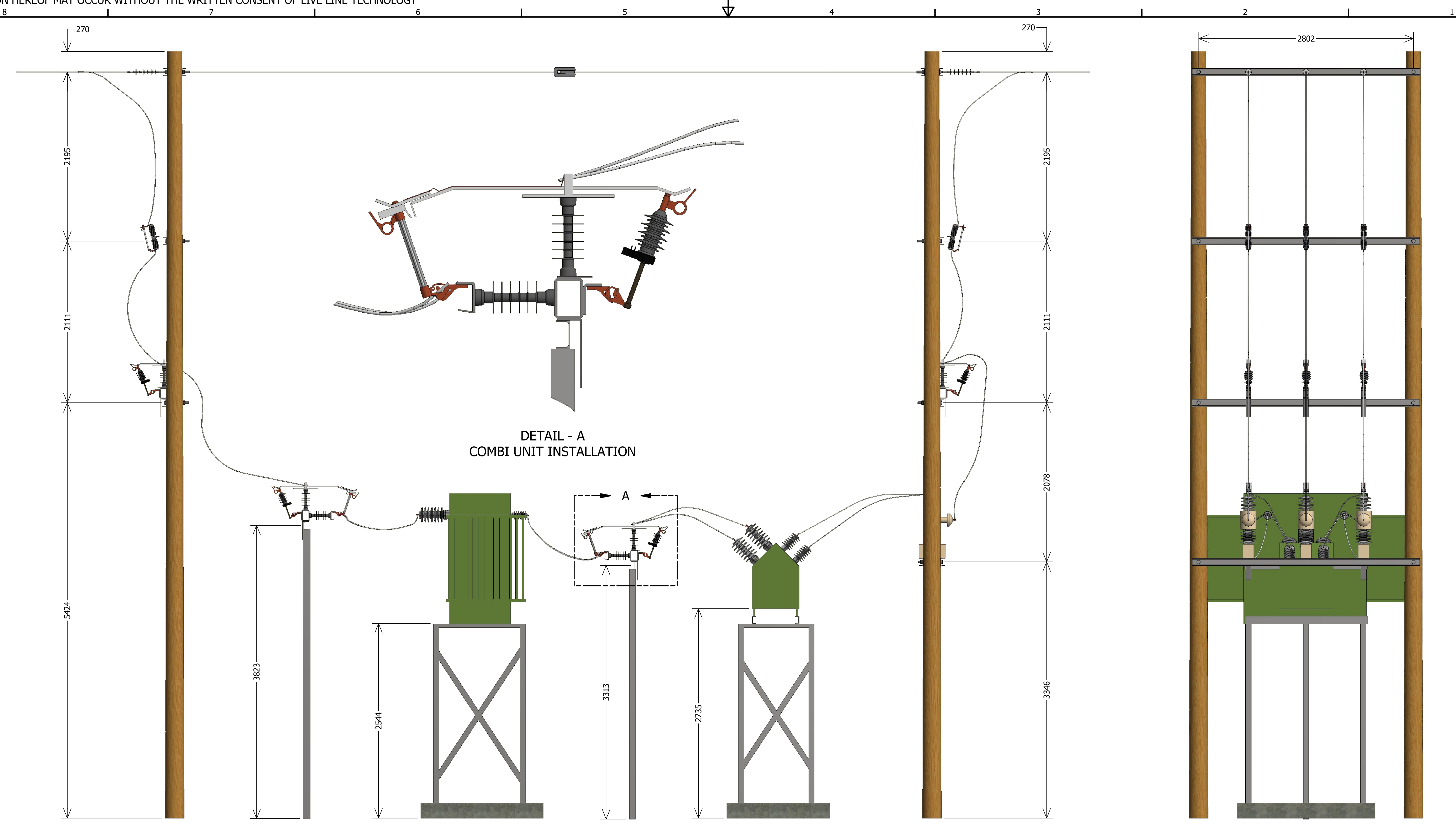
SIDE VIEW
